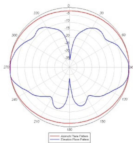
Figure 2: Azimuth and Elevation Plane Patterns for 5 GHz
